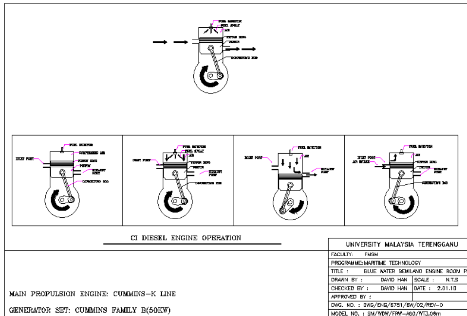
FIGURE 4: Mechanism of CI diesel propulsion engine in Gemilang 1
