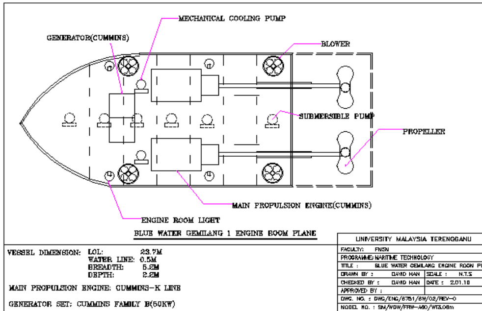
FIGURE 3: Machinery arrangement in Gemilang 1 engine room
